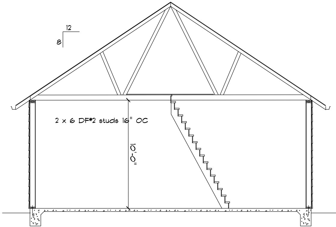
Traditional with Storage Cross Section 26ft wide
