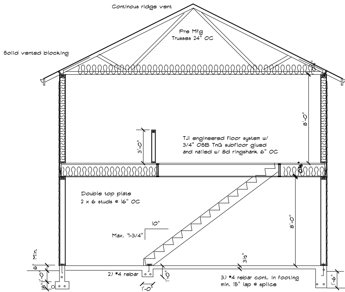
Homesteader Cross section AA 1/4" = 1'-0"
