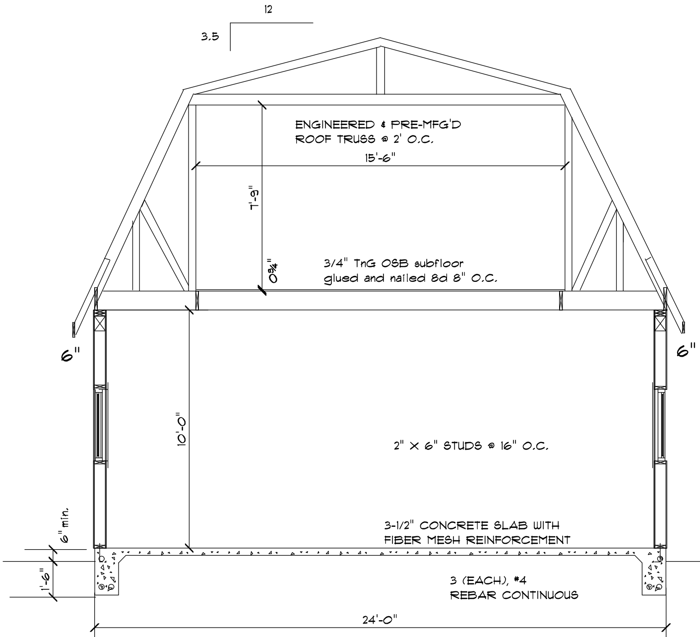
Gambrel Style Room in the Roof Cross Section
