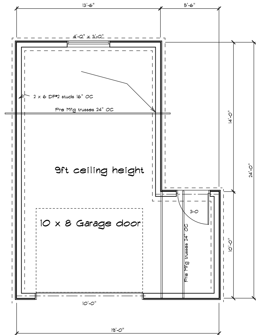
Floor plan
