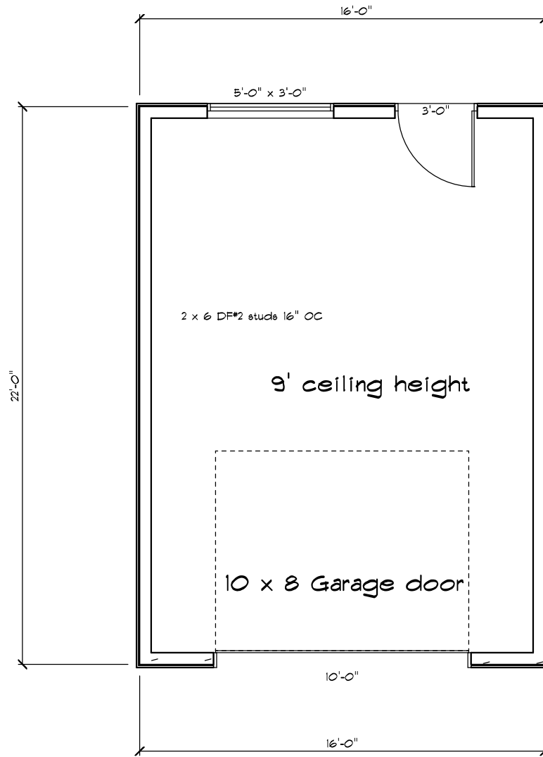
Floor plan
