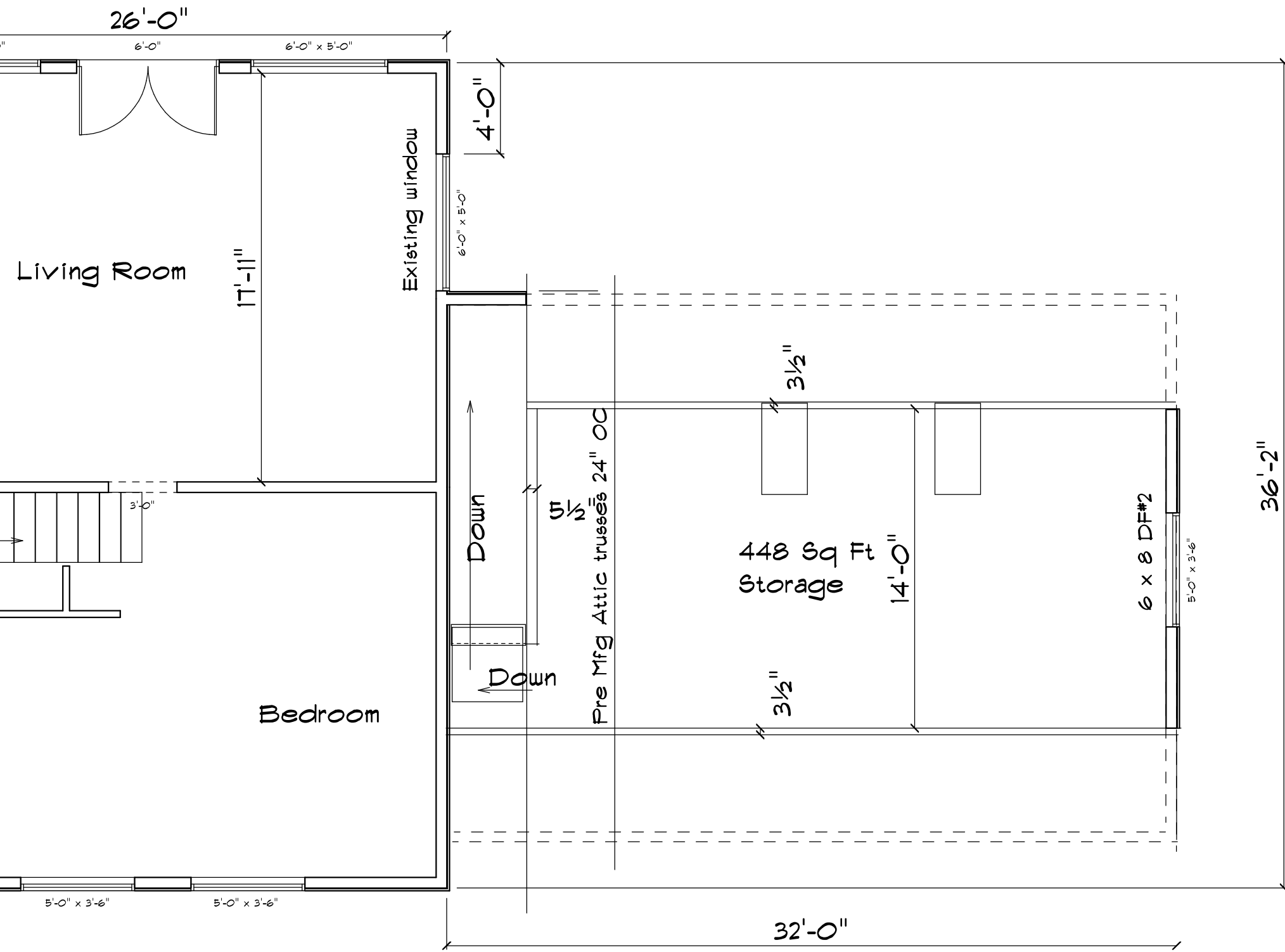
Loft Floorplan
