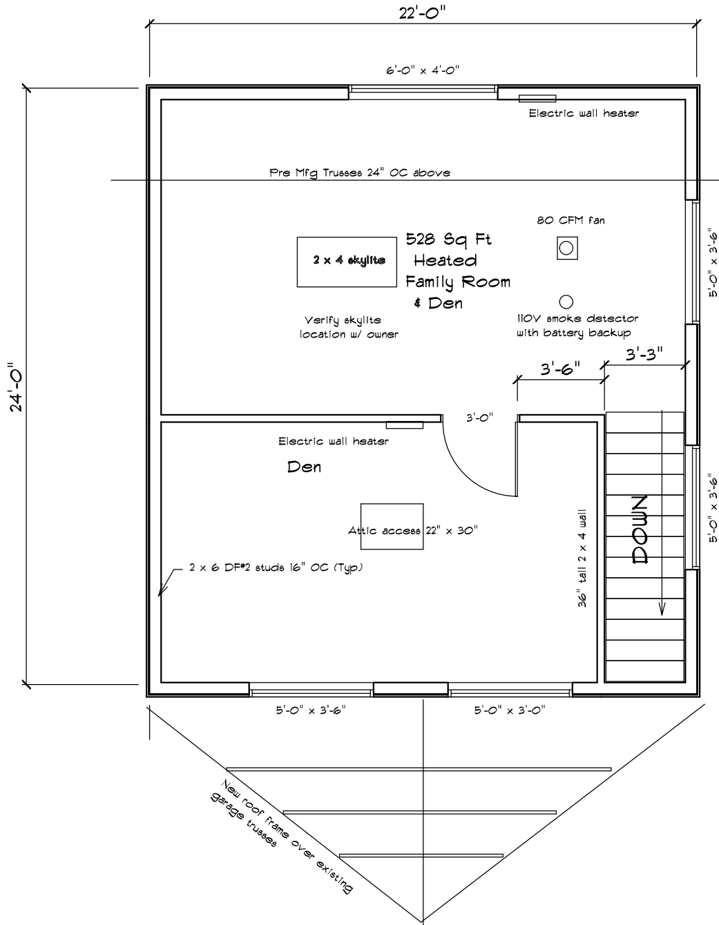
Second Floorplan
