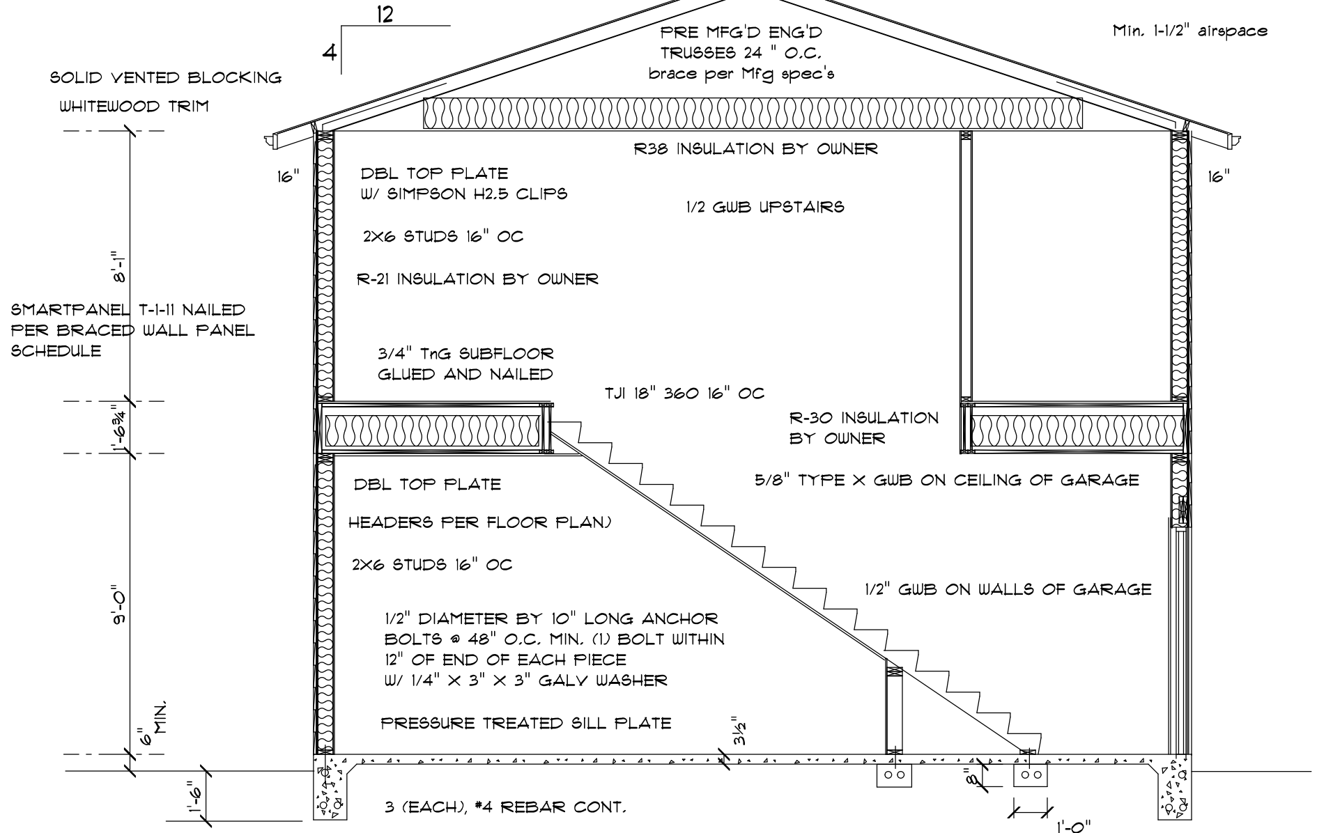
CROSS SECTION 1/4" = 1'-0"
