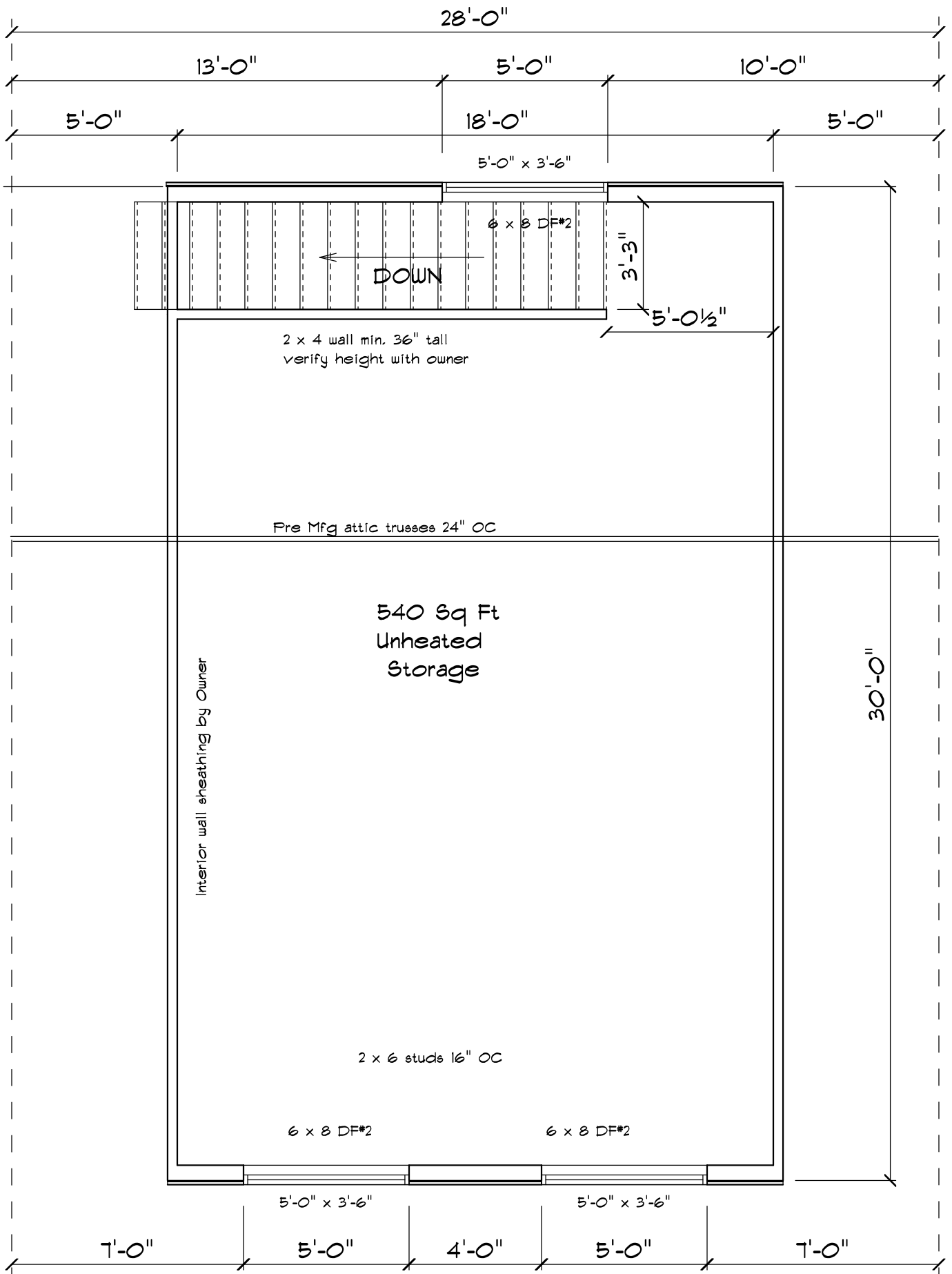
Second Floorplan 1/4" = 1'-0"
