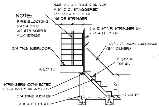
INTERIOR STAIR DETAIL
