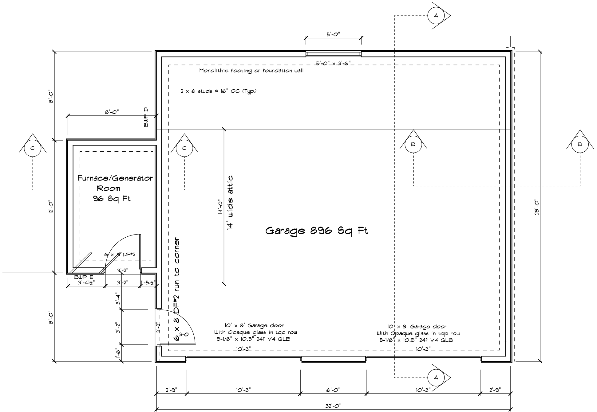
Garage Floorplan
