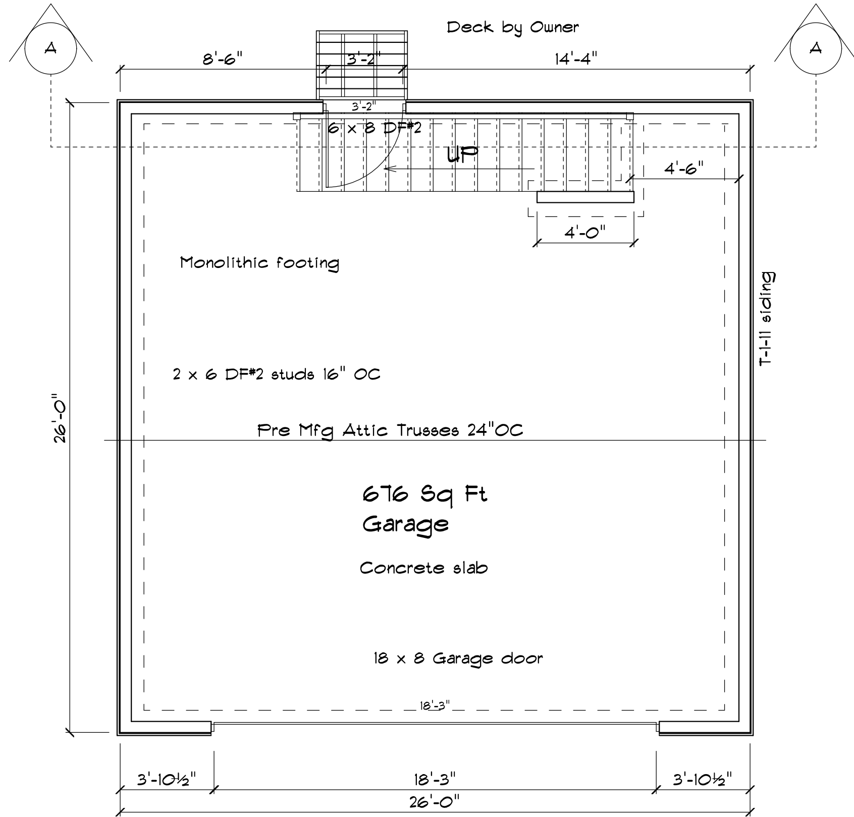
Garage Floorplan
