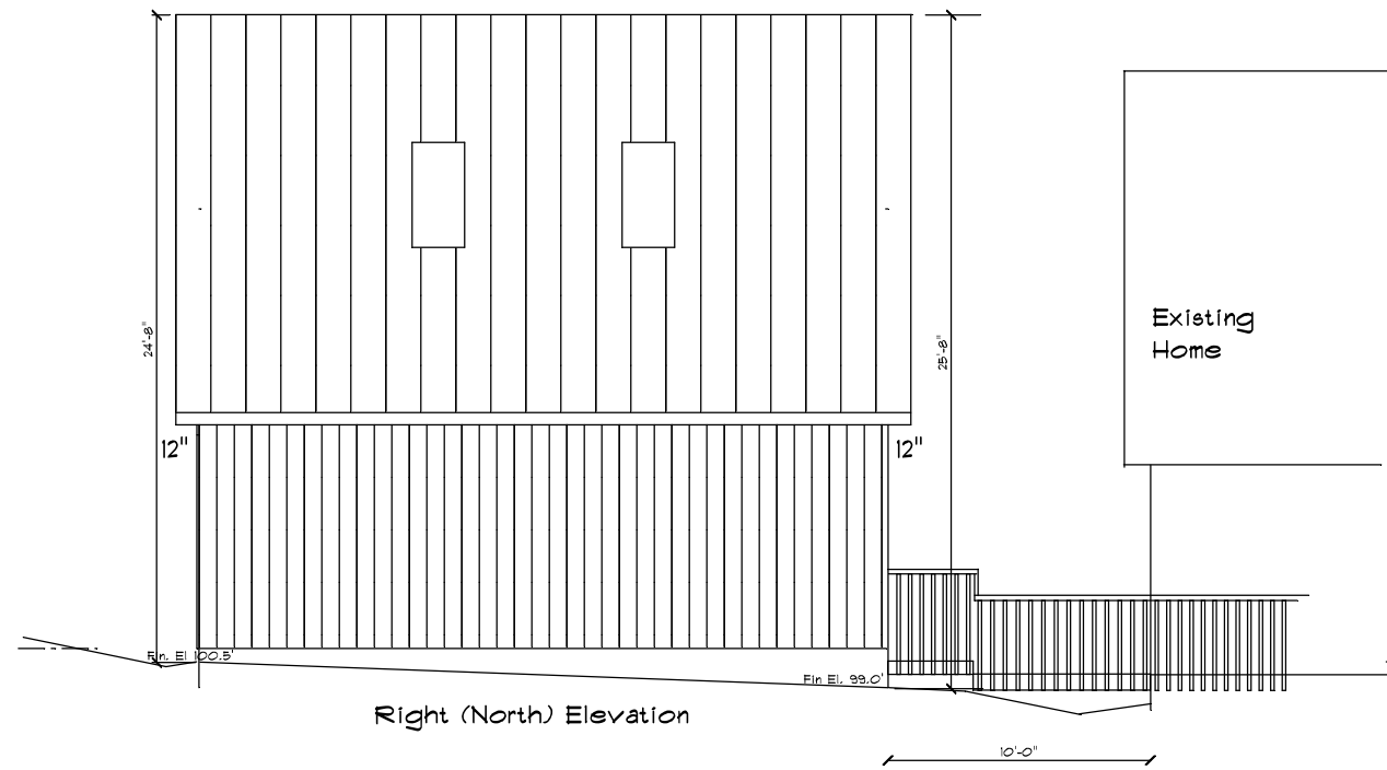
Right (North) Elevation
