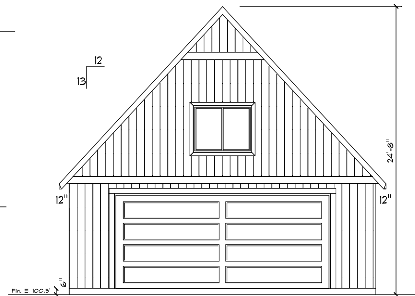
Front (East) Elevation 1/8" = 1'-0"
