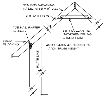
RAFTER OVER STAIRS DETAIL
