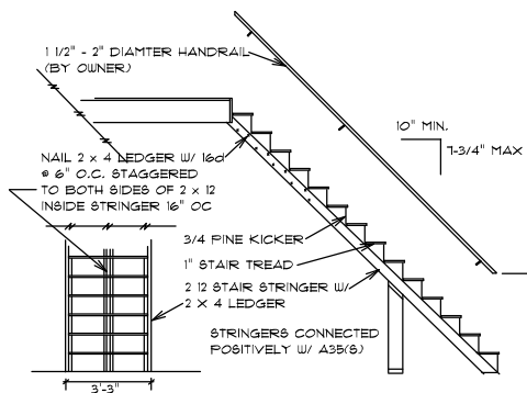
INTERIOR STAIR DETAIL
