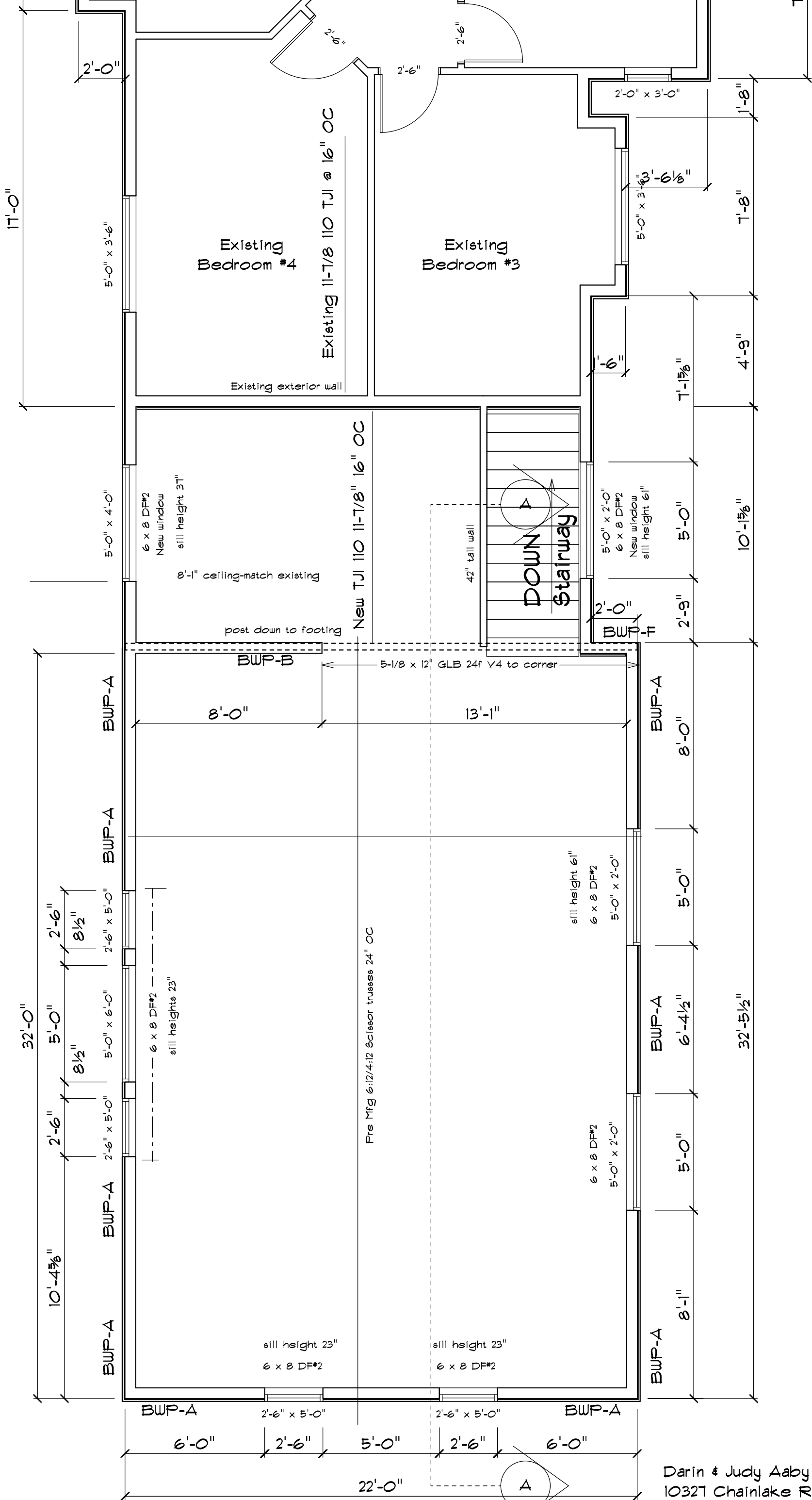
Second floorplan 1/4" = 1'-0"
